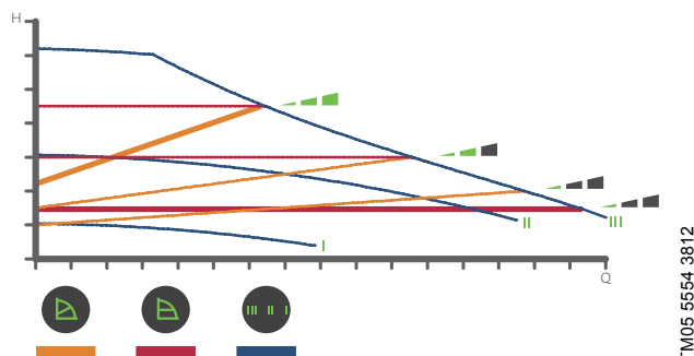
Fig. 22 Selection of pump setting for system type
