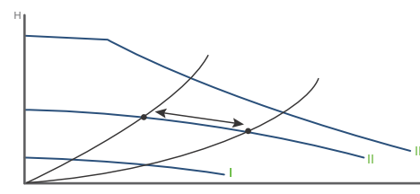
Fig. 25 Three constant-curve settings
