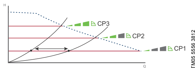
Fig. 24 Three constant-pressure curves/settings
